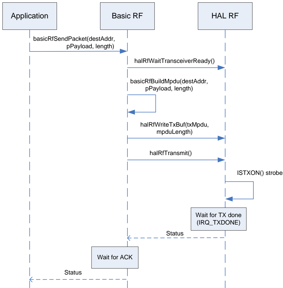
Figure 9 Packet transmission
