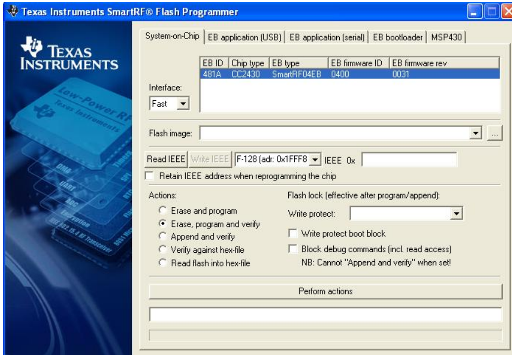
Figure 3 Flash Programmer
